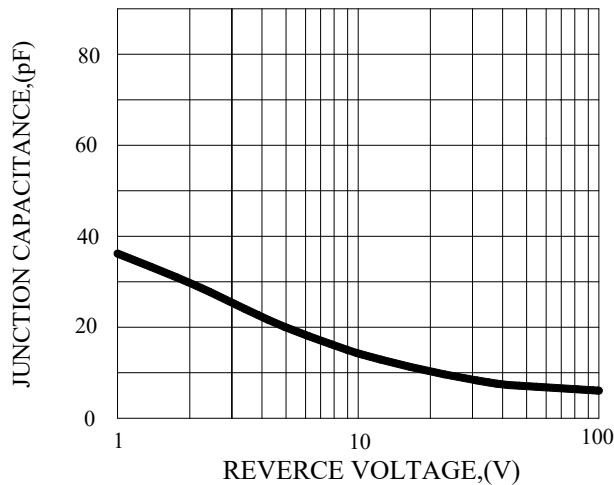
FIG.6-TYPICAL JUNCTION CAPACITANCE
